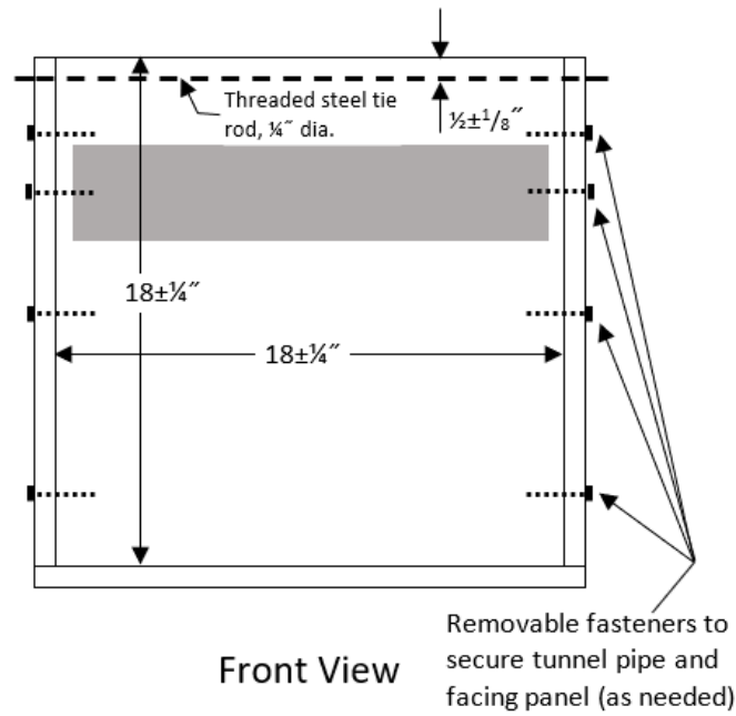
Figure 2: Sandbox dimensions (not to scale)
