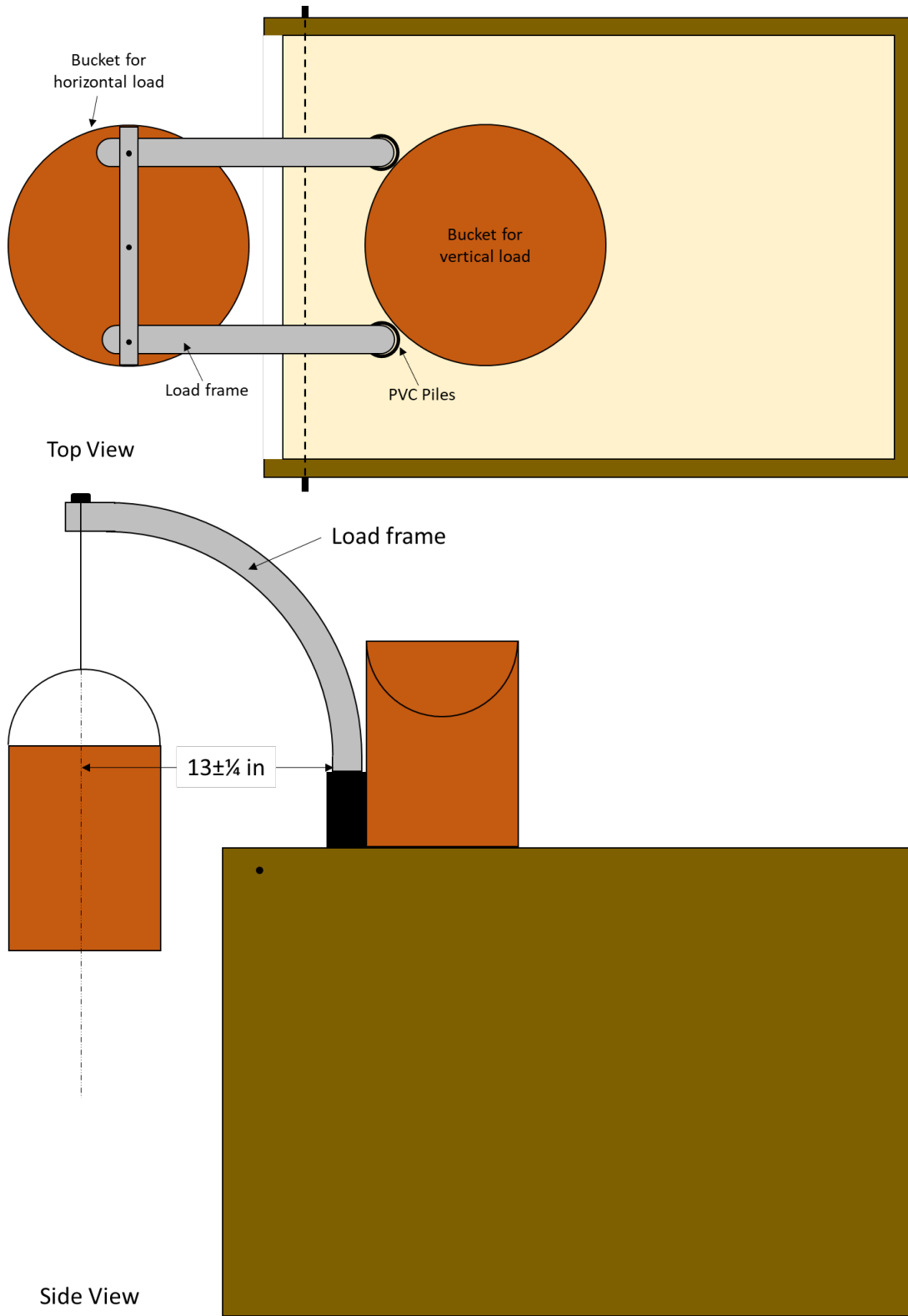
Figure 5: Load Placement (not to scale)
